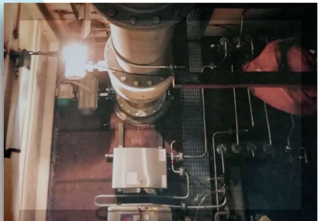
Ballast Treatment Plant Installation.
